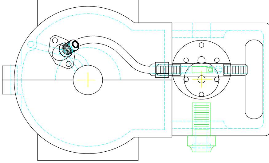
Rear View of Crankcase Shows oil pipes and fittings
