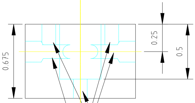
Pump Body Side View
